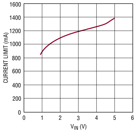
Current Limit vs V_{IN} Voltage
